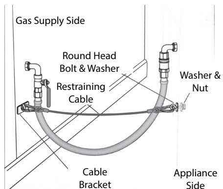
Restraining Cable
