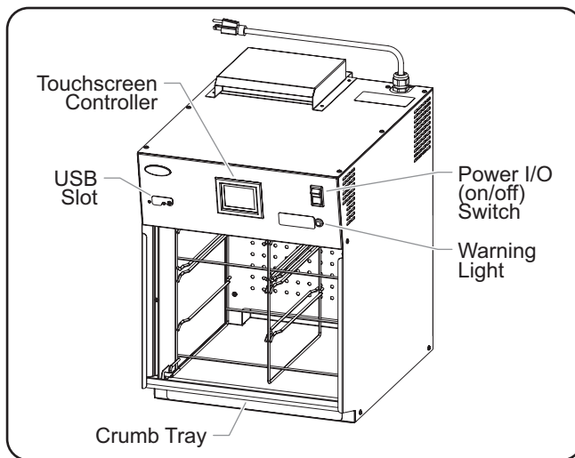
Model FS2HAC-15
