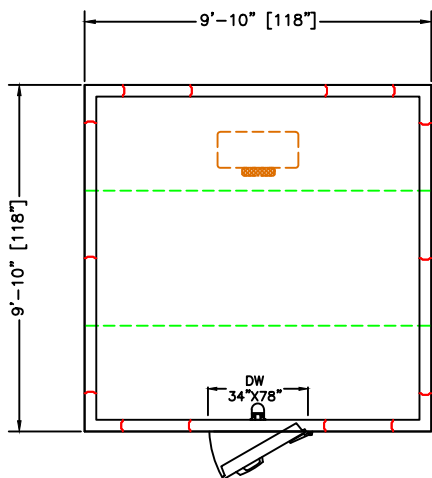
PLAN VIEW
