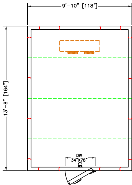
PLAN VIEW
