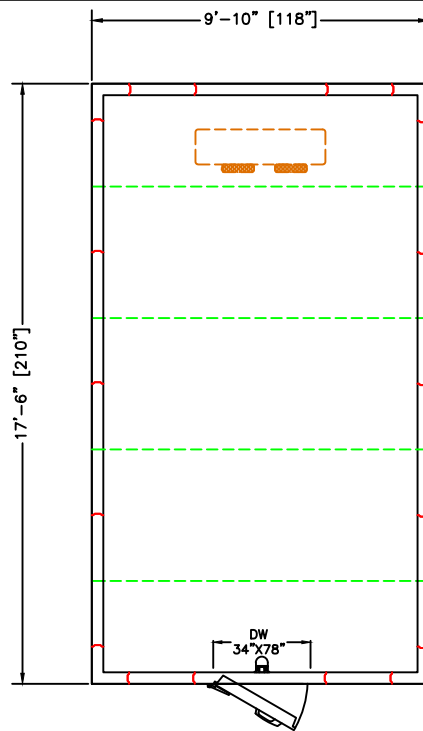
PLAN VIEW LEFT HINGE SELECT
