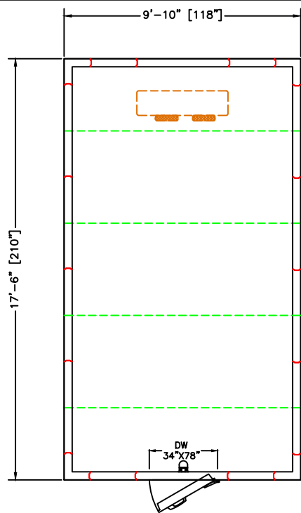
PLAN VIEW RIGHT HINGE SELECT
