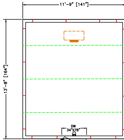
PLAN VIEW LEFT HINGE SELECT
