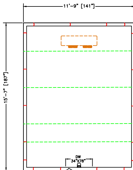
PLAN VIEW LEFT HINGE SELECT
