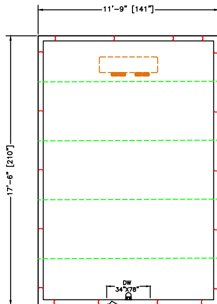
PLAN VIEW LEFT HINGE SELECT
