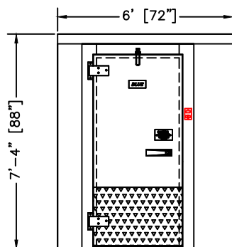
ELEVATION LEFT HINGE
