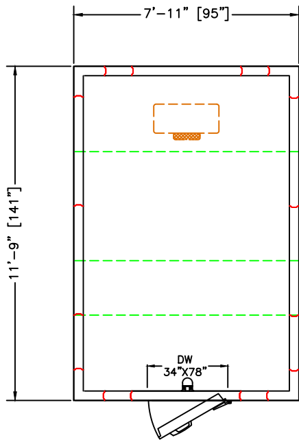
PLAN VIEW
