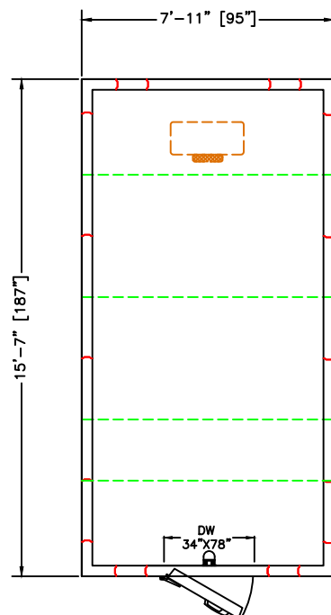
PLAN VIEW LEFT HINGE SELECT
