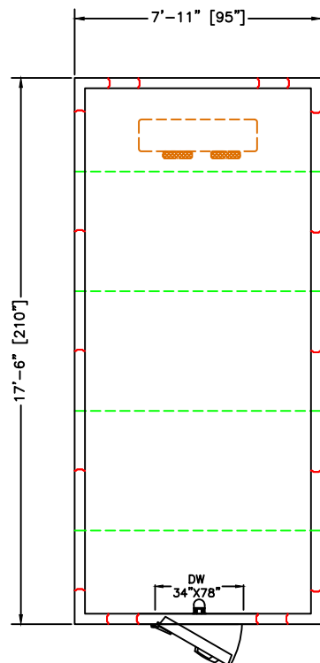
PLAN VIEW
