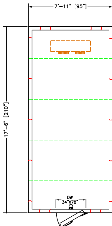
PLAN VIEW
