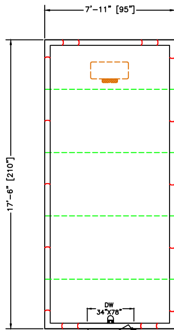
PLAN VIEW RIGHT HINGE SELECT
