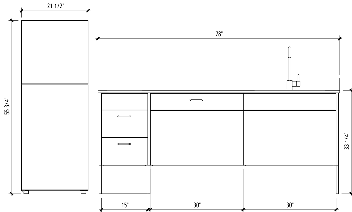
① CABINET ELEVATION 3/4" = 1'-0"
