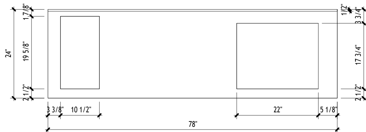
③ COUNTERTOP PLAN 3/4" = 1'-0"
